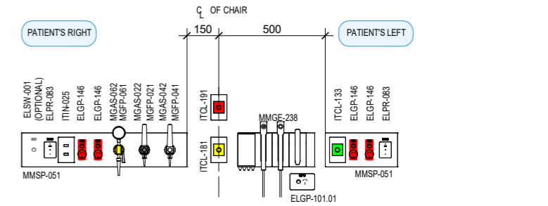
DETAIL MSP 1 (1:25 @ A3)
