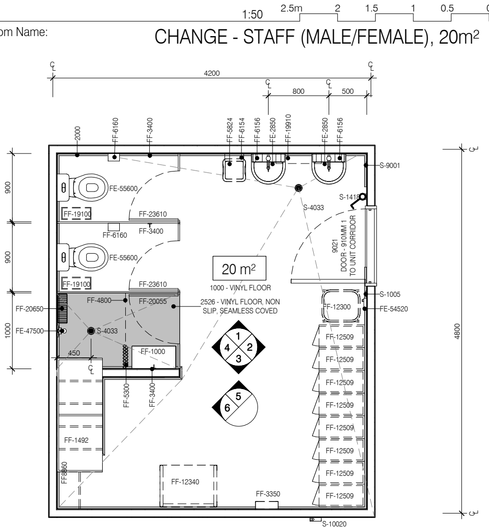
PLAN
