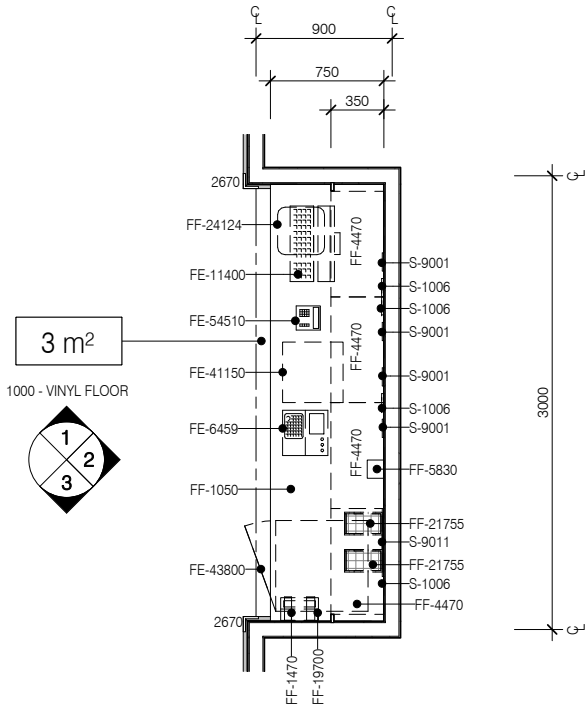
PLAN
