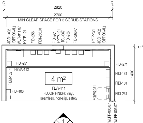
PLAN
