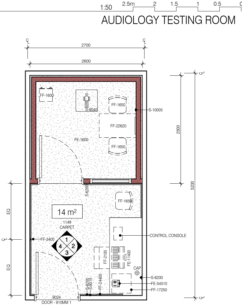
PLAN
