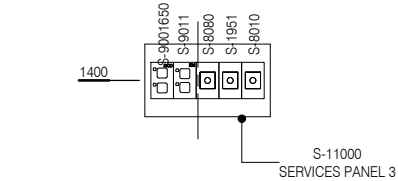
ELEVATION 7 ( 1 : 25 @ A3 )
