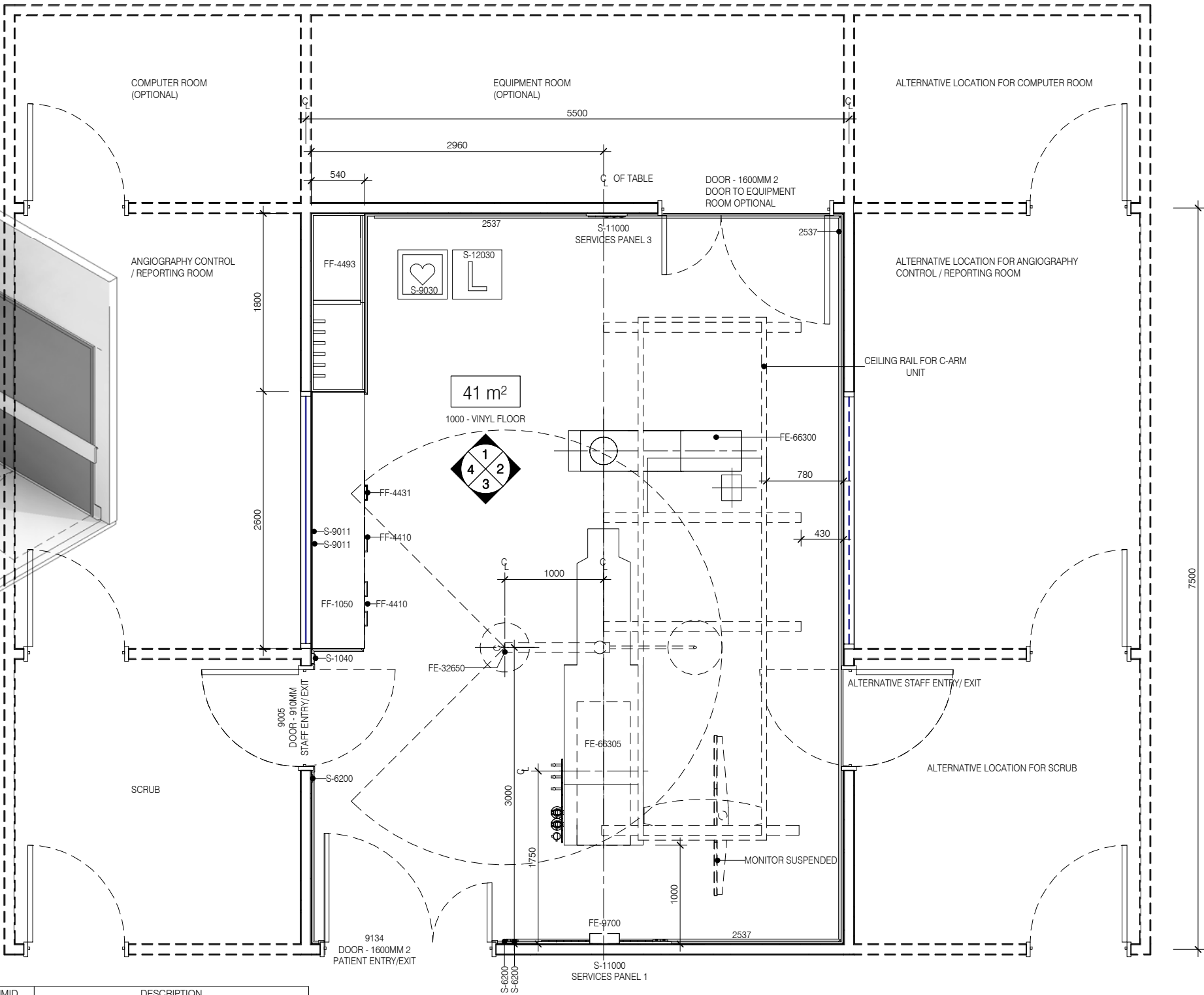
PLAN
