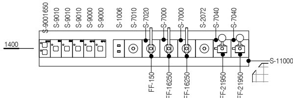
ELEVATION 5 ( 1 : 25 @ A3 )
