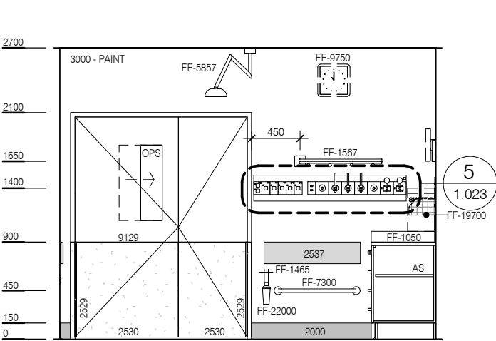
ELEVATION 5 ( 1 : 25 @ A3 )
