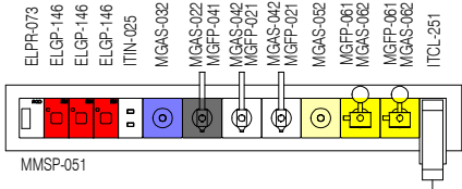
ELEVATION 5 ( 1 : 25 @ A3 )
