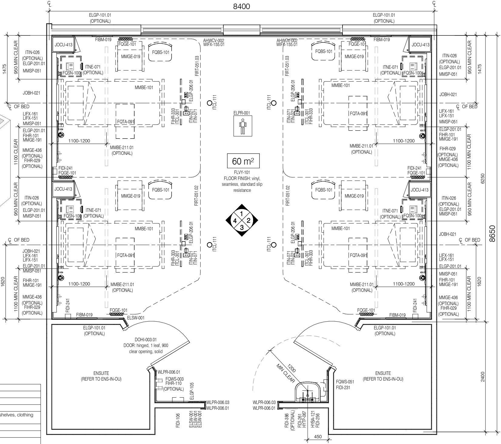
PLAN
