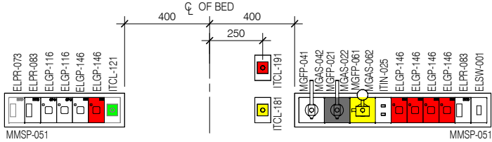
DETAIL M1 - MSP 1 (1:25 @ A3)
