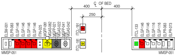
DETAIL M2 - MSP 2 (1:25 @ A3)
