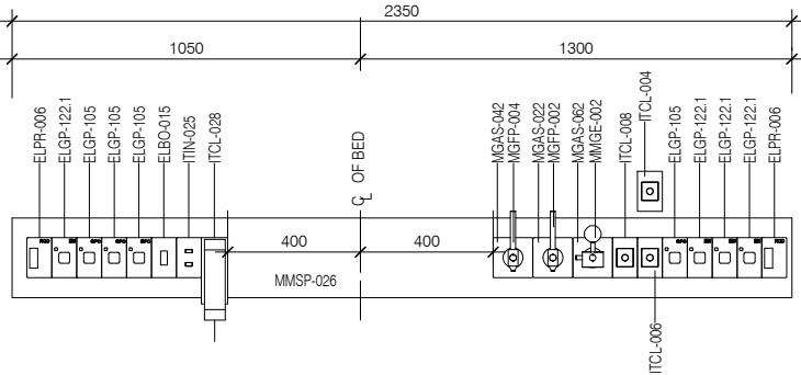
ELEVATION 5 ( 1 : 25 @ A3 )
