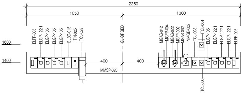
ELEVATION 5 ( 1 : 25 @ A3 )
