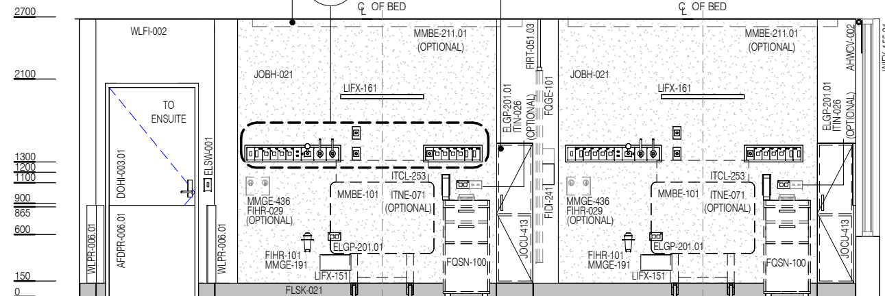
OPTIONAL. PROVISION OF A LIFTING TRACK IS TO BE CONFIRMED AT PROJECT LEVEL TO SUIT CLINICAL SERVICE REQUIREMENTS AND LOCAL WHS POLICIES FOR PATIENT HANDLING. CONFIGURATION, INSTALLATION (CEILING MOUNTED OR RECESSED), WEIGHT RATING/SAFE WORKING LOAD (SWL) REQUIREMENTS, AND EXTENT MUST ALSO BE CONSIDERED AND CONFIRMED BY PROJECT TEAMS. SELECTED EQUIPMENT IS TO MEET LOCAL IPSC POLICIES AND CLEANING REQUIREMENTS. REQUIREMENTS FOR LOADING AND STORAGE OF PATIENT LIFTER MOTOR/CASSETTE IS TO BE CONFIRMED TO SUIT CLINICAL SERVICE REQUIREMENTS AND OPERATIONAL MODELS
