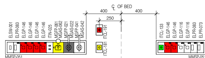
MSP DETAIL ( 1 : 25 @ A3 )
