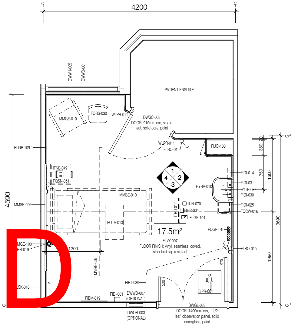
PLAN
