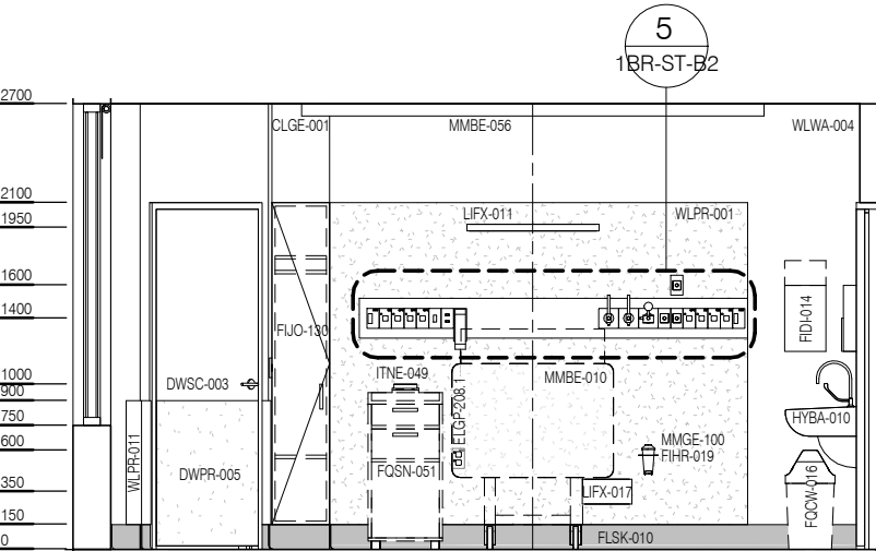
ELEVATION 5 ( 1 : 25 @ A3 )
