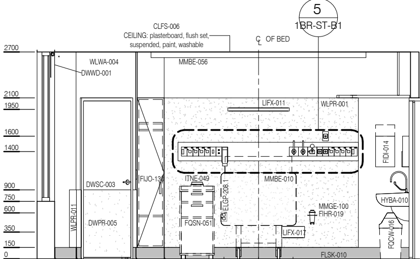
ELEVATION 5 ( 1 : 25 @ A3 )
