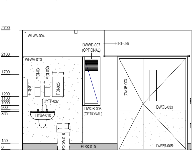
ELEVATION 5 ( 1 : 25 @ A3 )
