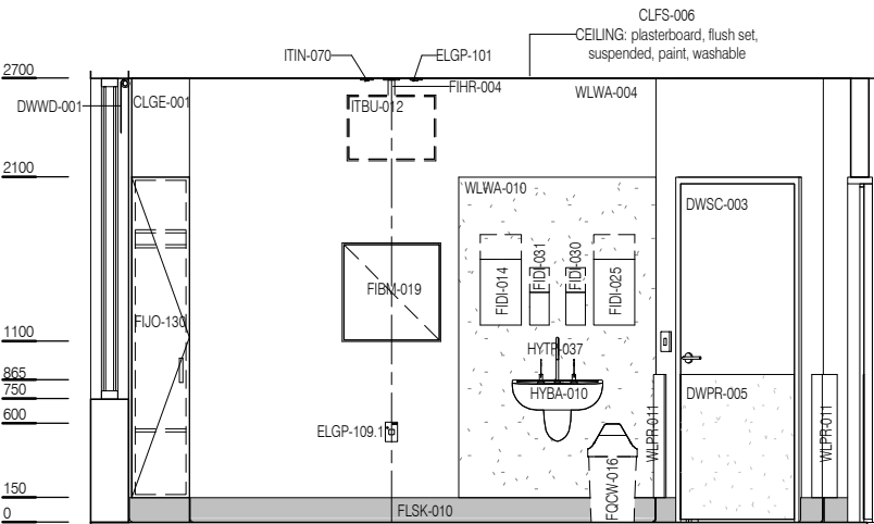
ELEVATION 5 ( 1 : 25 @ A3 )
