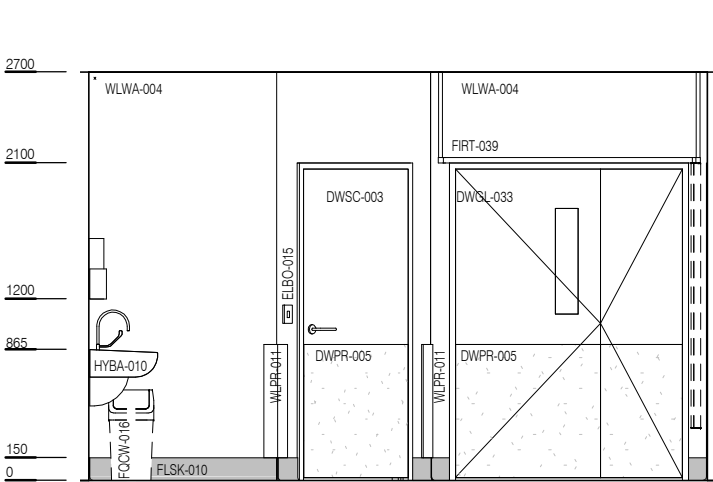
ELEVATION 5 ( 1 : 25 @ A3 )
