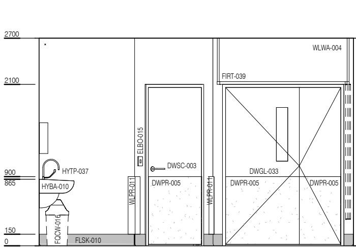
ELEVATION 5 ( 1 : 25 @ A3 )
