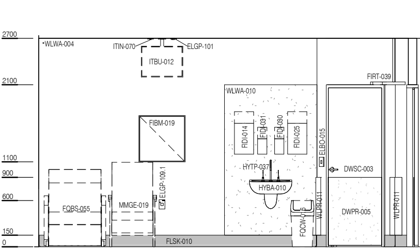
ELEVATION 5 ( 1 : 25 @ A3 )
