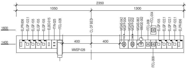
ELEVATION 5 ( 1 : 25 @ A3 )
