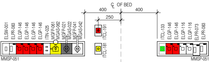
MSP DETAIL ( 1 : 25 @ A3 )
