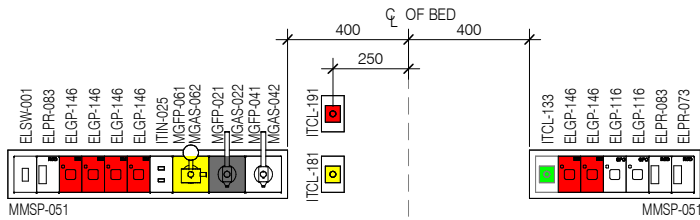
MSP DETAIL ( 1 : 25 @ A3 )
