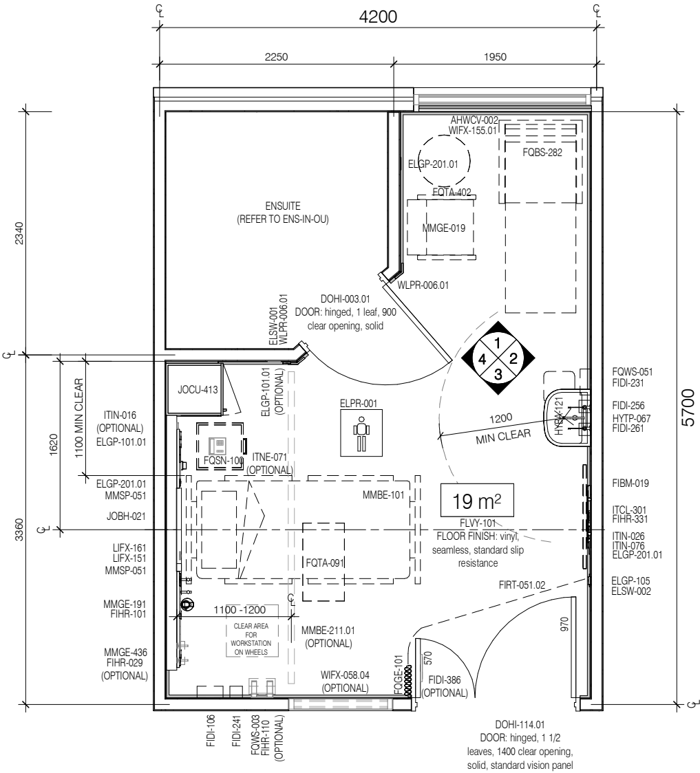
PLAN
