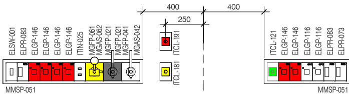
MSP DETAIL ( 1 : 25 @ A3 )
