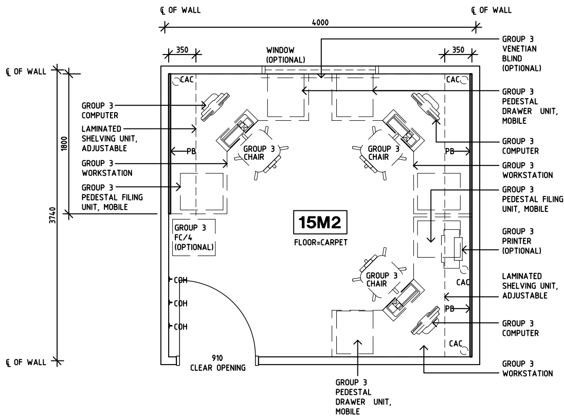
PLAN
