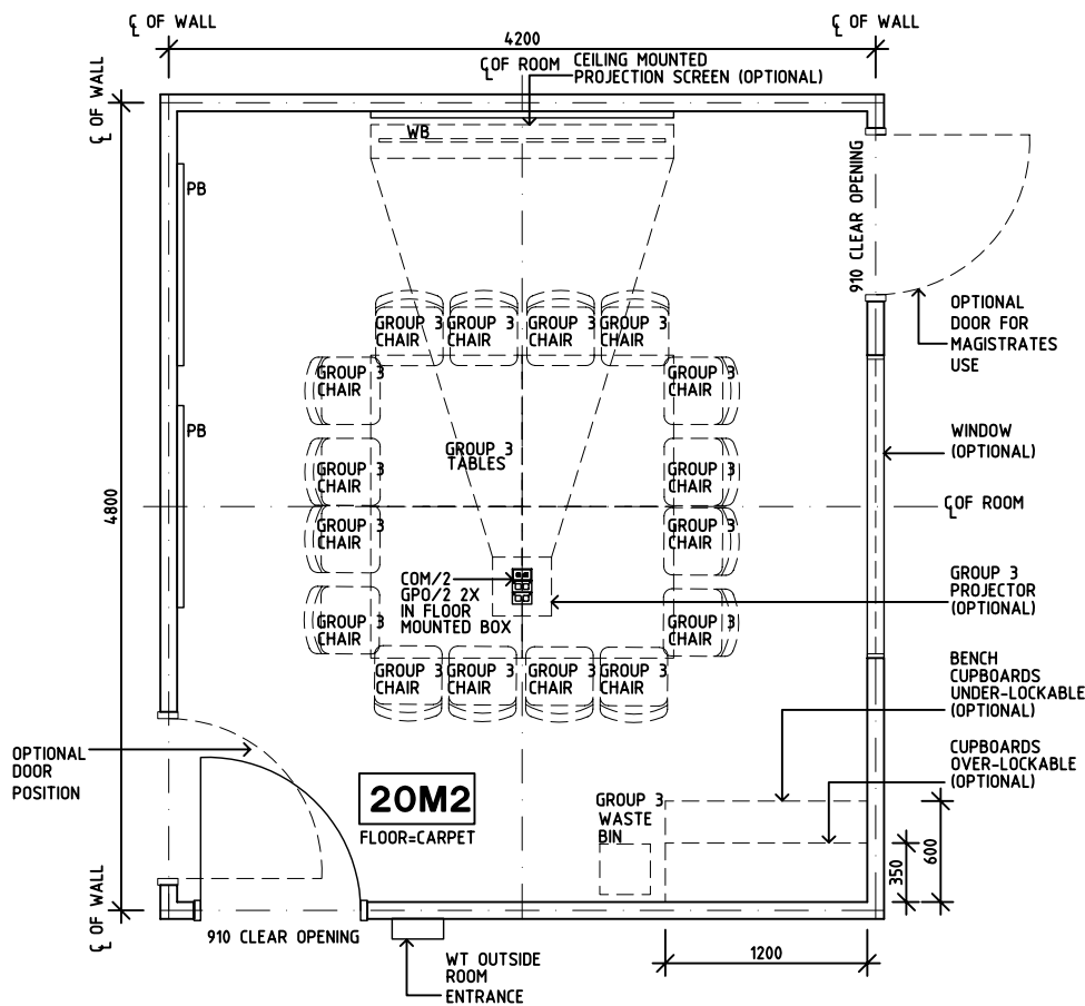
PLAN
