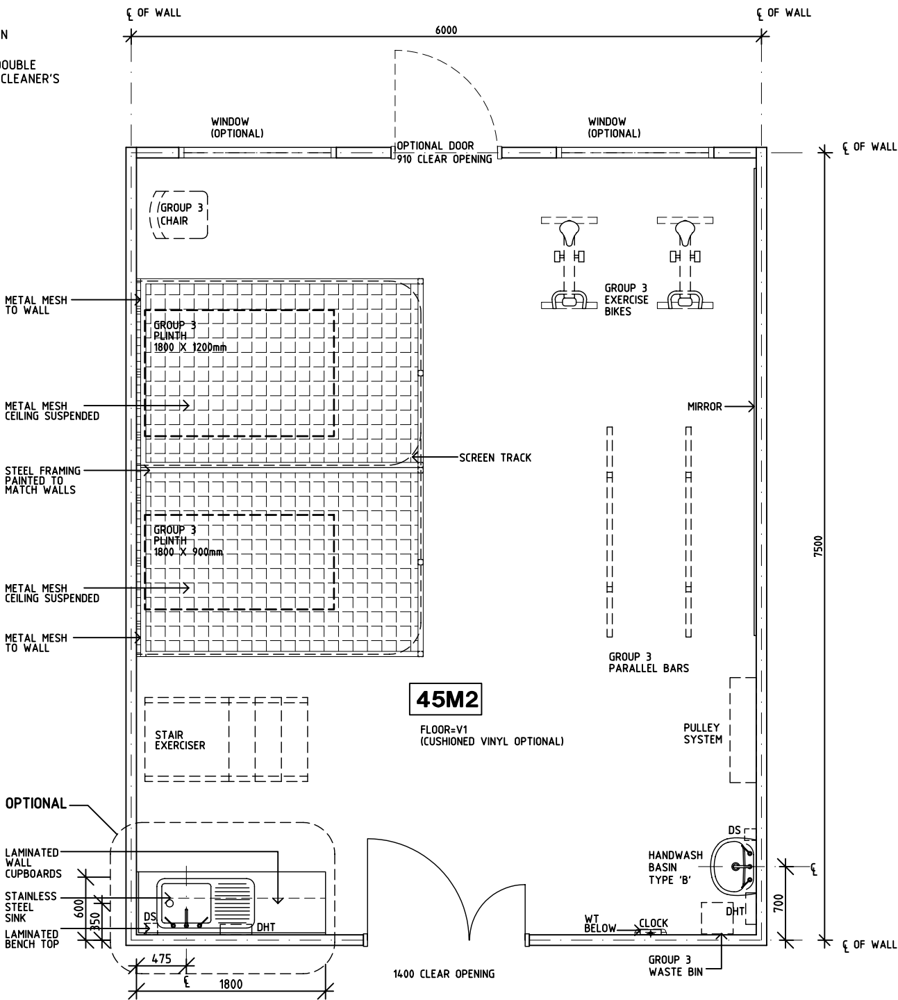
PLAN
